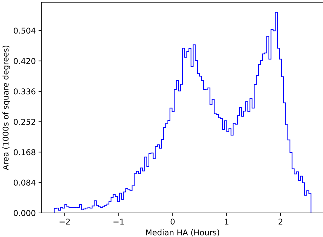
start_date_do-180v3.4_10yrs All sky u band: Median HA
