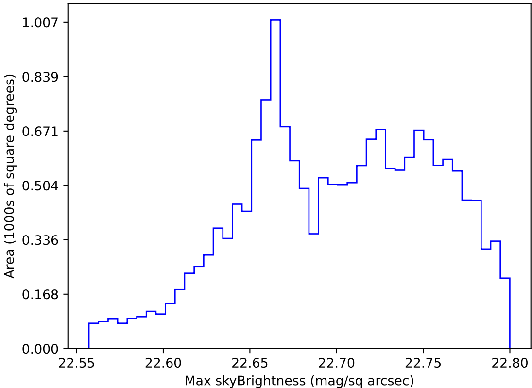
start_date_do-180v3.4_10yrs WFD u band: Max skyBrightness
