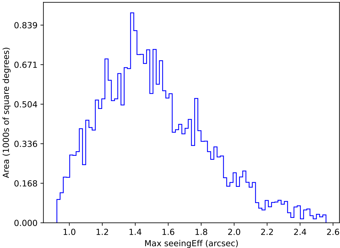
start_date_do-180v3.4_10yrs Yr 1 z band: Max seeingEff
