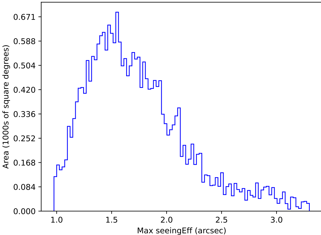
start_date_do-180v3.4_10yrs Yr 1 u band: Max seeingEff
