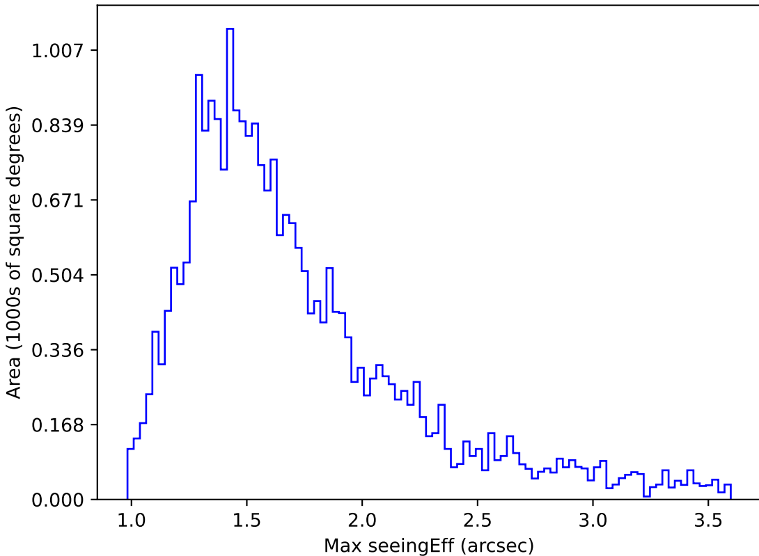
start_date_do-180v3.4_10yrs Yr 1 g band: Max seeingEff
