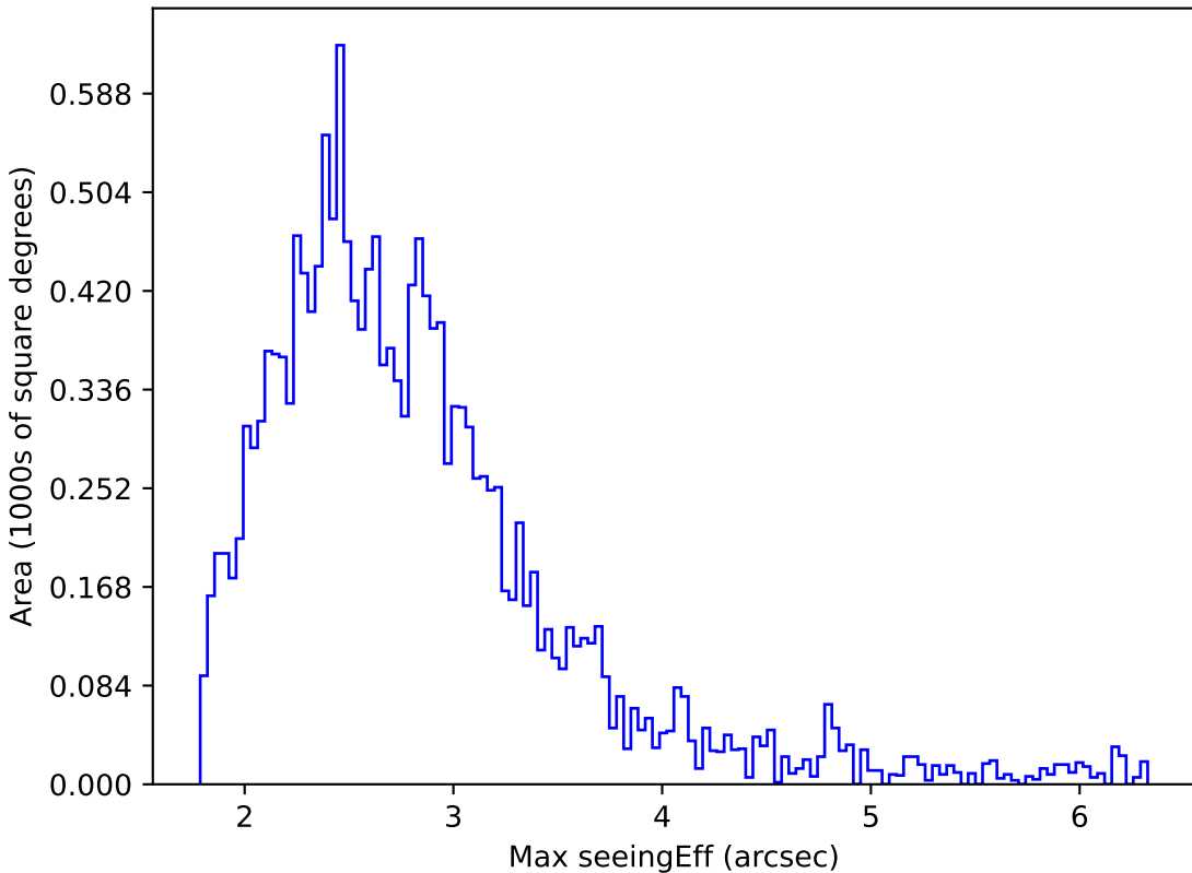
start_date_do-180v3.4_10yrs WFD r band: Max seeingEff
