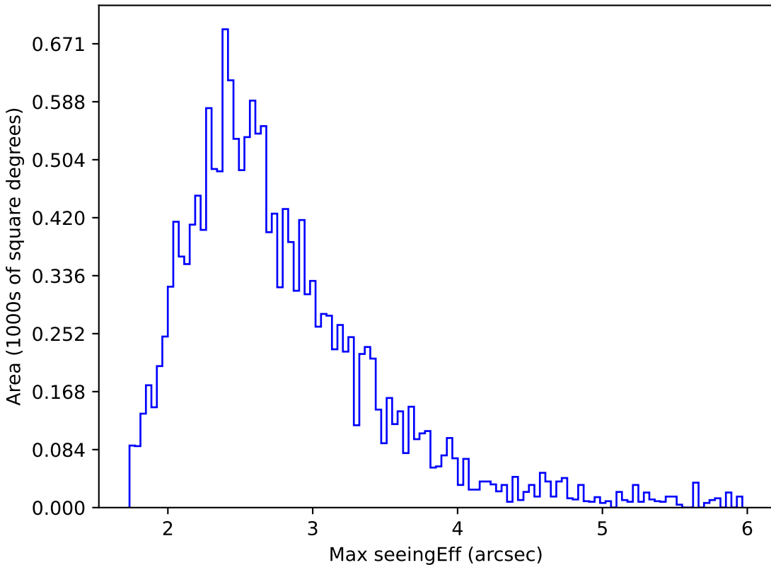
start_date_do-180v3.4_10yrs WFD i band: Max seeingEff
