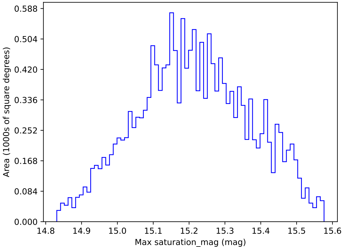
start_date_do-180v3.4_10yrs WFD z band: Max saturation_mag
