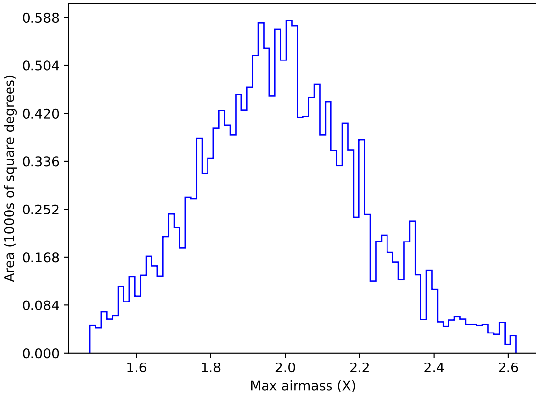
start_date_do-180v3.4_10yrs WFD g band: Max airmass
