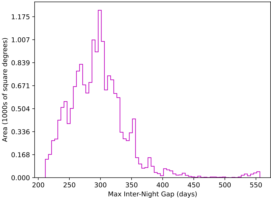
start_date_do-180v3.4_10yrs WFD z band: Max Inter-Night Gap
