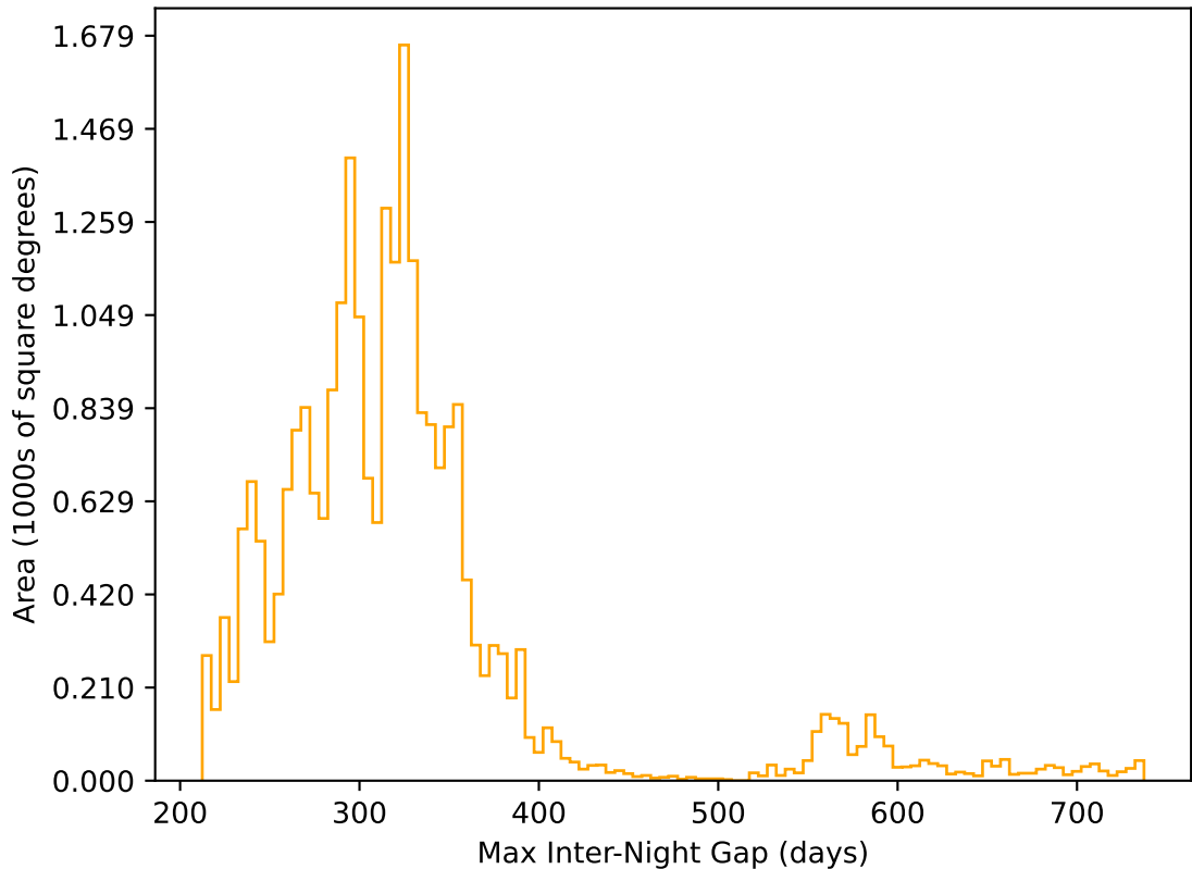
start_date_do-180v3.4_10yrs All sky r band: Max Inter-Night Gap
