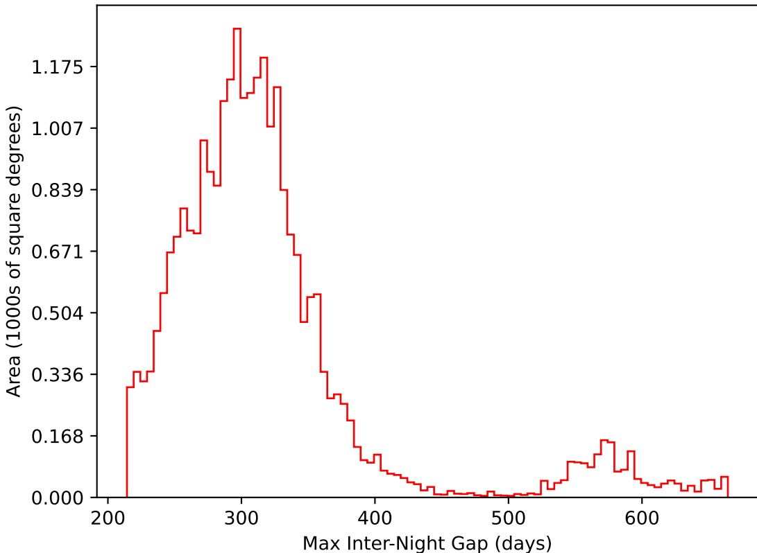
start_date_do-180v3.4_10yrs All sky i band: Max Inter-Night Gap
