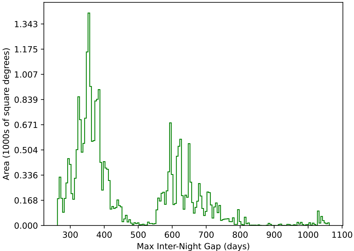
start_date_do-180v3.4_10yrs All sky g band: Max Inter-Night Gap
