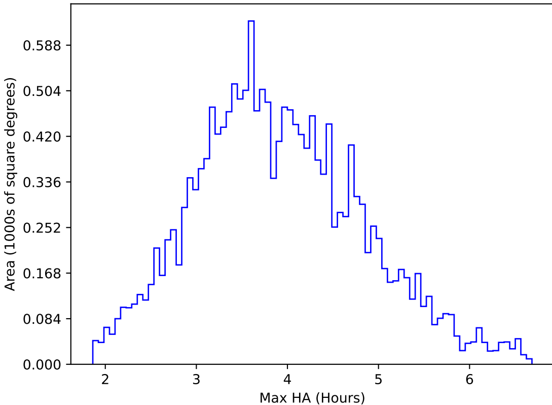
start_date_do-180v3.4_10yrs WFD u band: Max HA
