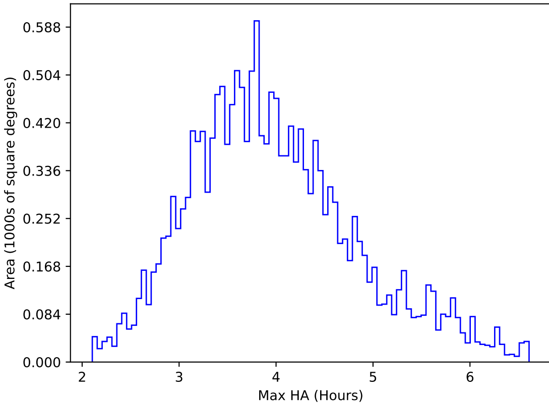
start_date_do-180v3.4_10yrs WFD g band: Max HA
