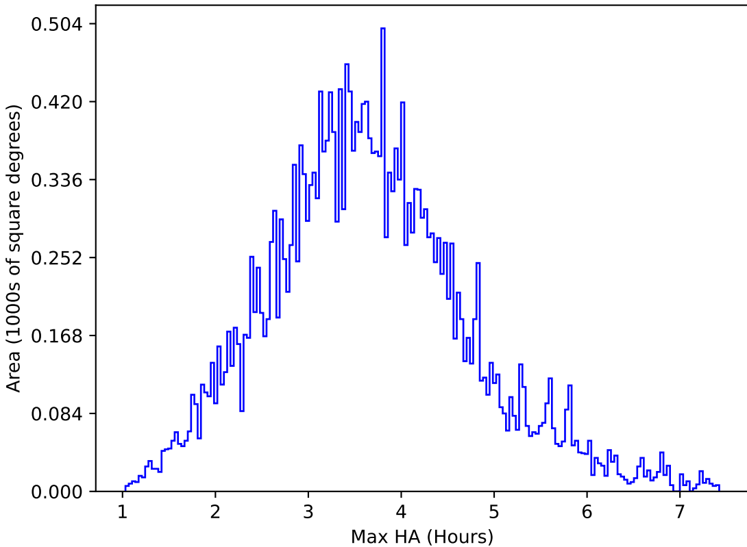
start_date_do-180v3.4_10yrs All sky g band: Max HA
