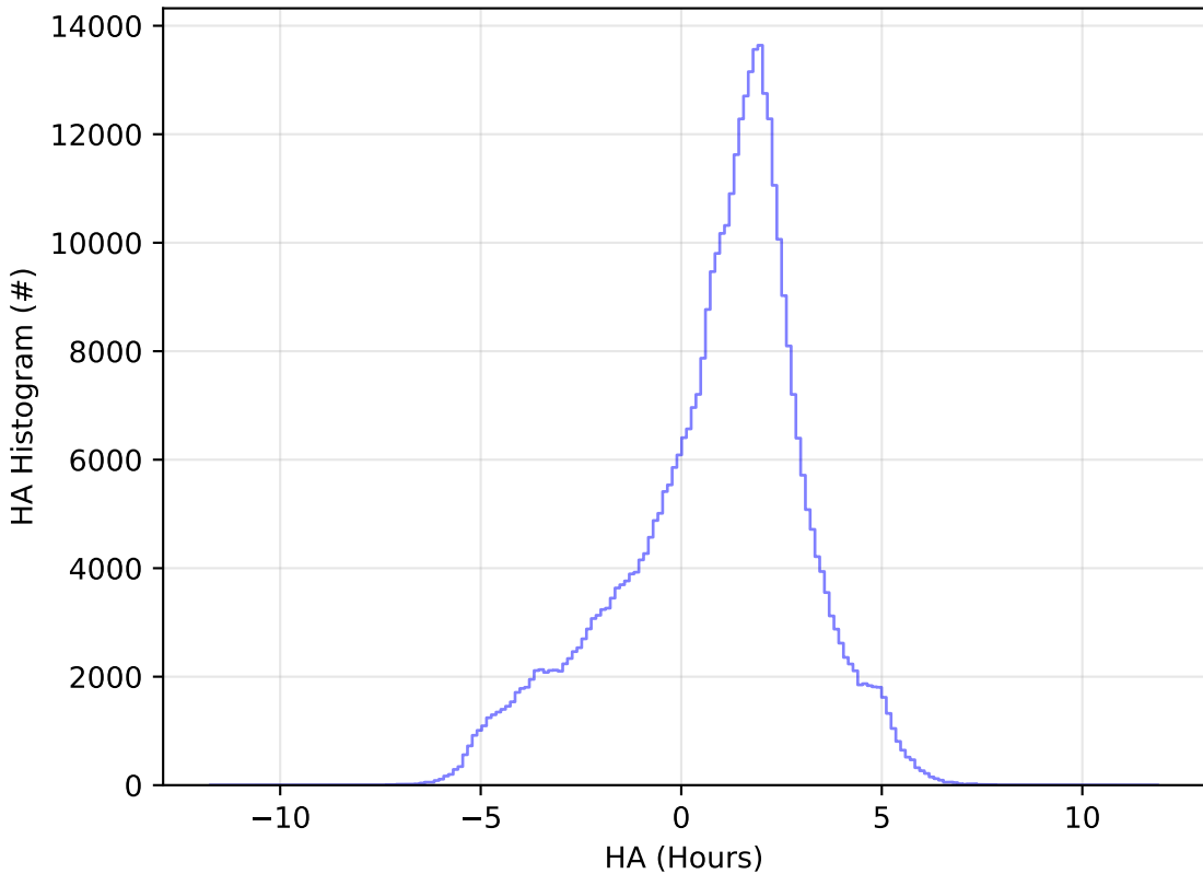
start_date_do-180v3.4_10yrs WFD z band: HA Histogram
