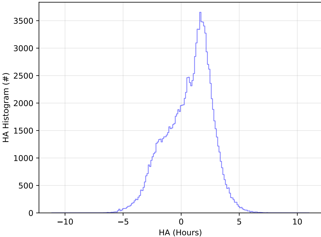
start_date_do-180v3.4_10yrs WFD u band: HA Histogram
