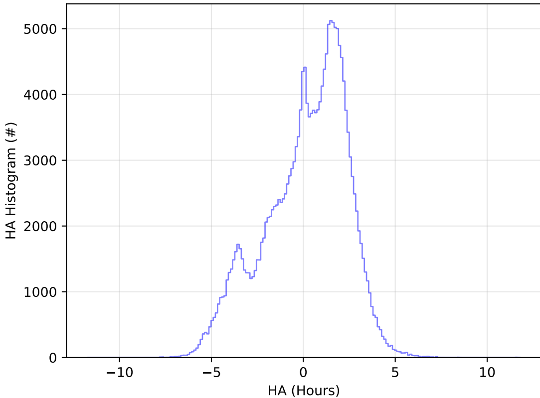
start_date_do-180v3.4_10yrs WFD g band: HA Histogram
