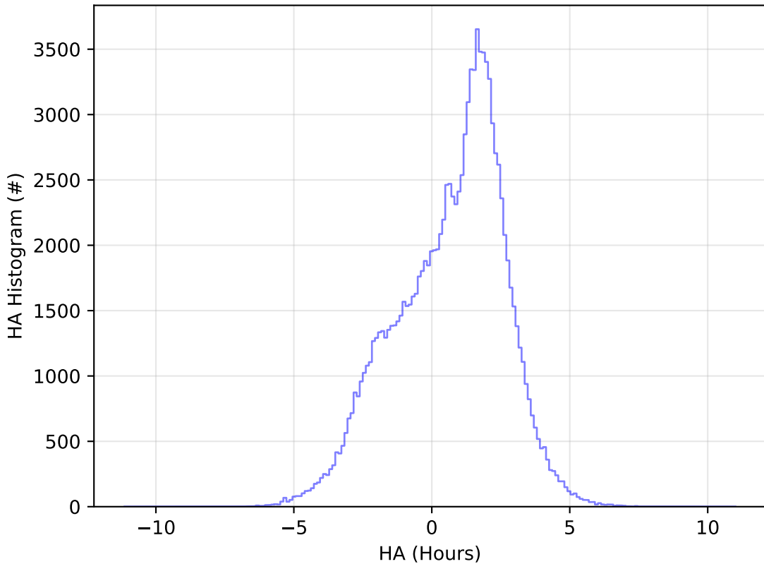
start_date_do-180v3.4_10yrs All sky u band: HA Histogram
