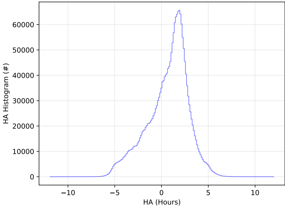
start_date_do-180v3.4_10yrs All sky all bands: HA Histogram
