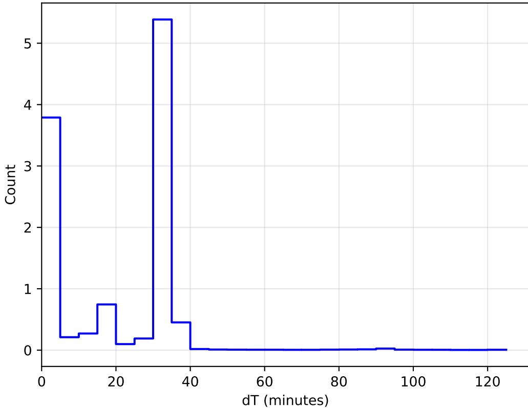
start_date_do-180v3.4_10yrs WFD: DeltaT Histogram
