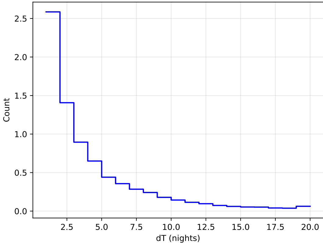
start_date_do-180v3.4_10yrs WFD all bands: DeltaNight Histogram 1e6
