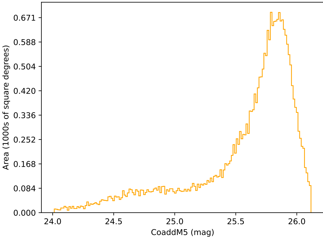
start_date_do-180v3.4_10yrs Yr 1 r band: CoaddM5
