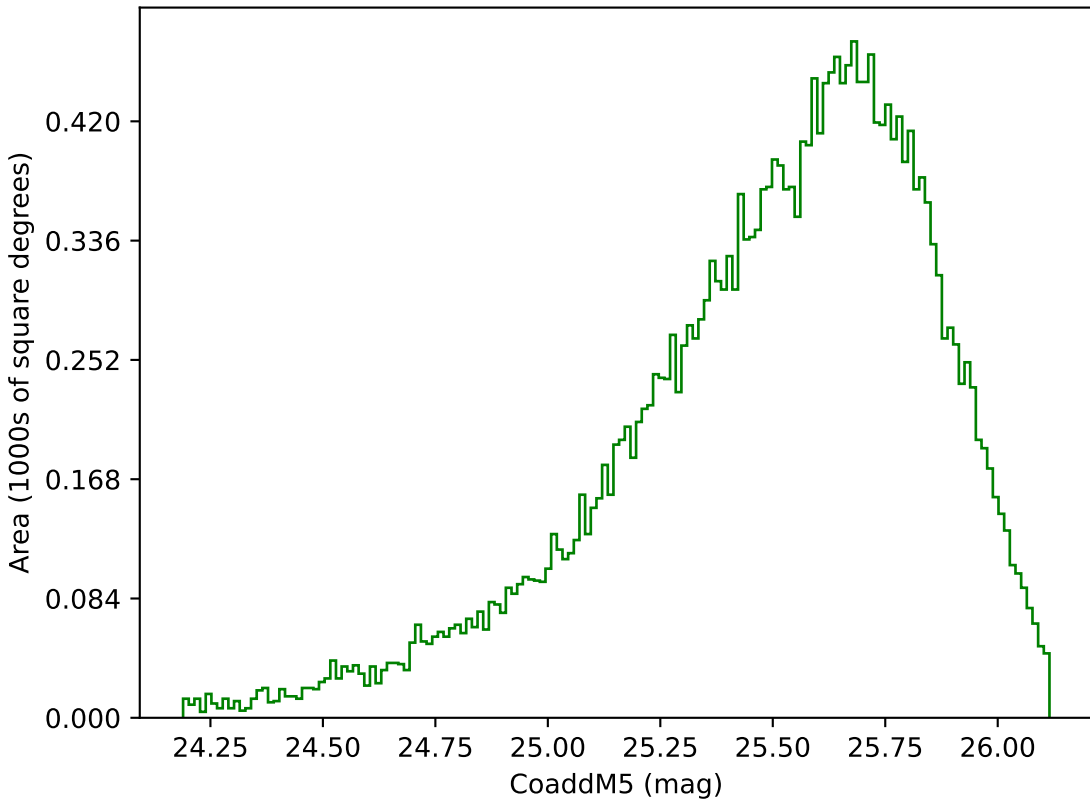
start_date_do-180v3.4_10yrs Yr 1 g band: CoaddM5
