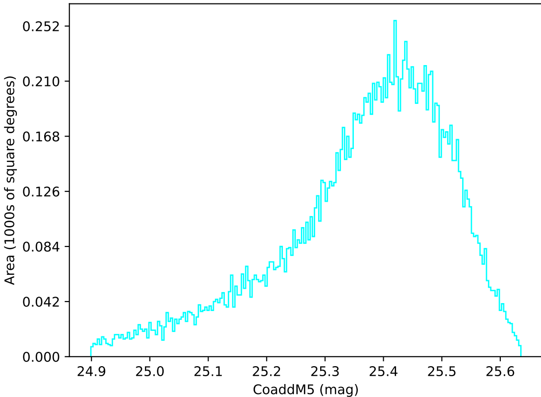
start_date_do-180v3.4_10yrs WFD u band: CoaddM5
