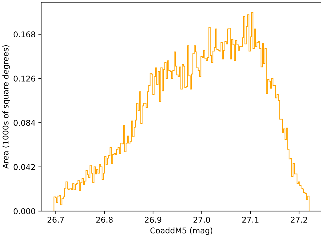
start_date_do-180v3.4_10yrs WFD r band: CoaddM5
