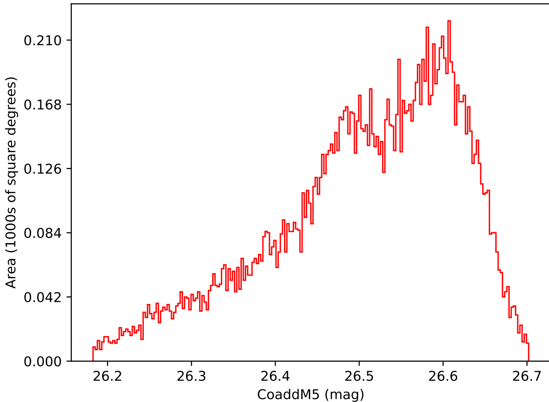
start_date_do-180v3.4_10yrs WFD i band: CoaddM5
