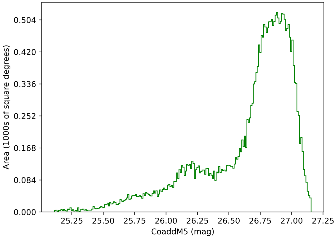
start_date_do-180v3.4_10yrs All sky g band: CoaddM5
