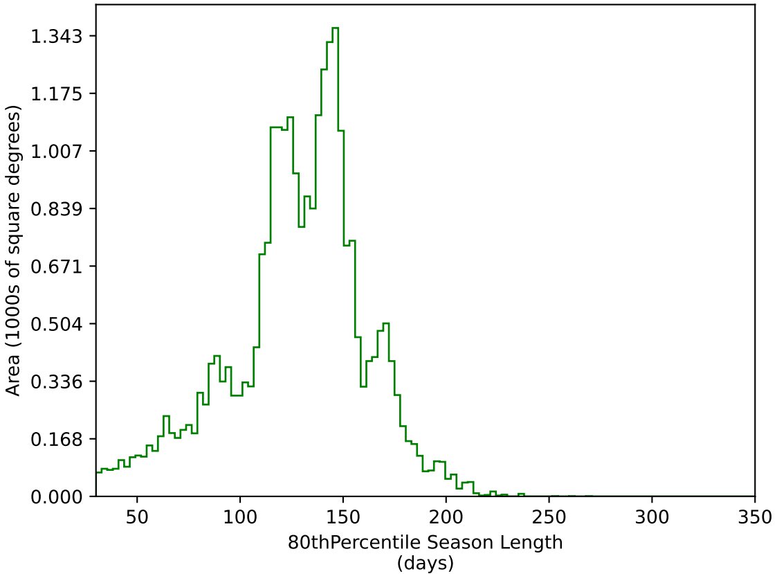
start_date_do-180v3.4_10yrs All sky g band: 80thPercentile Season Length
