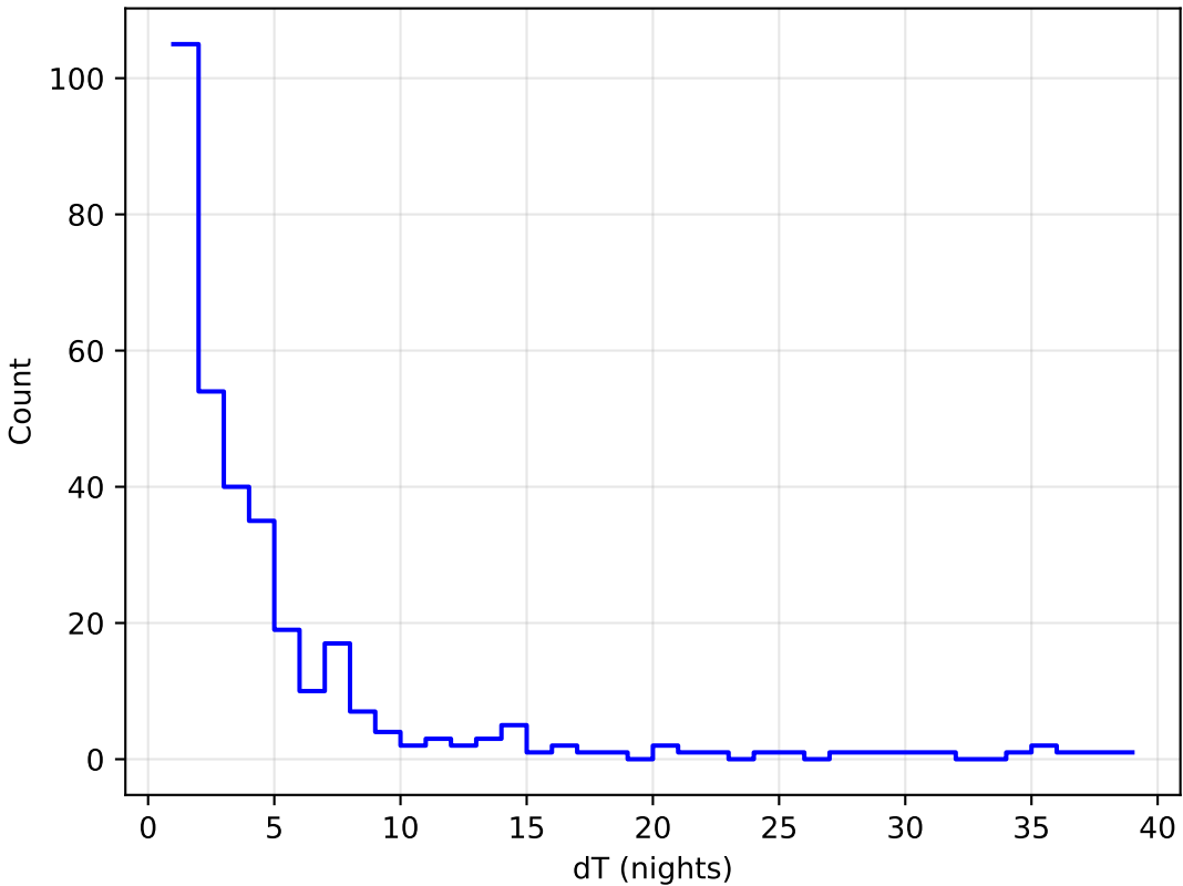
start_date_do-180v3.4_10yrs all bands: DD:WFD Delta Nights Histogram
