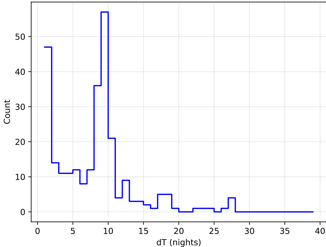
start_date_do-180v3.4_10yrs all bands: DD:ELAISS1 Delta Nights Histogram
