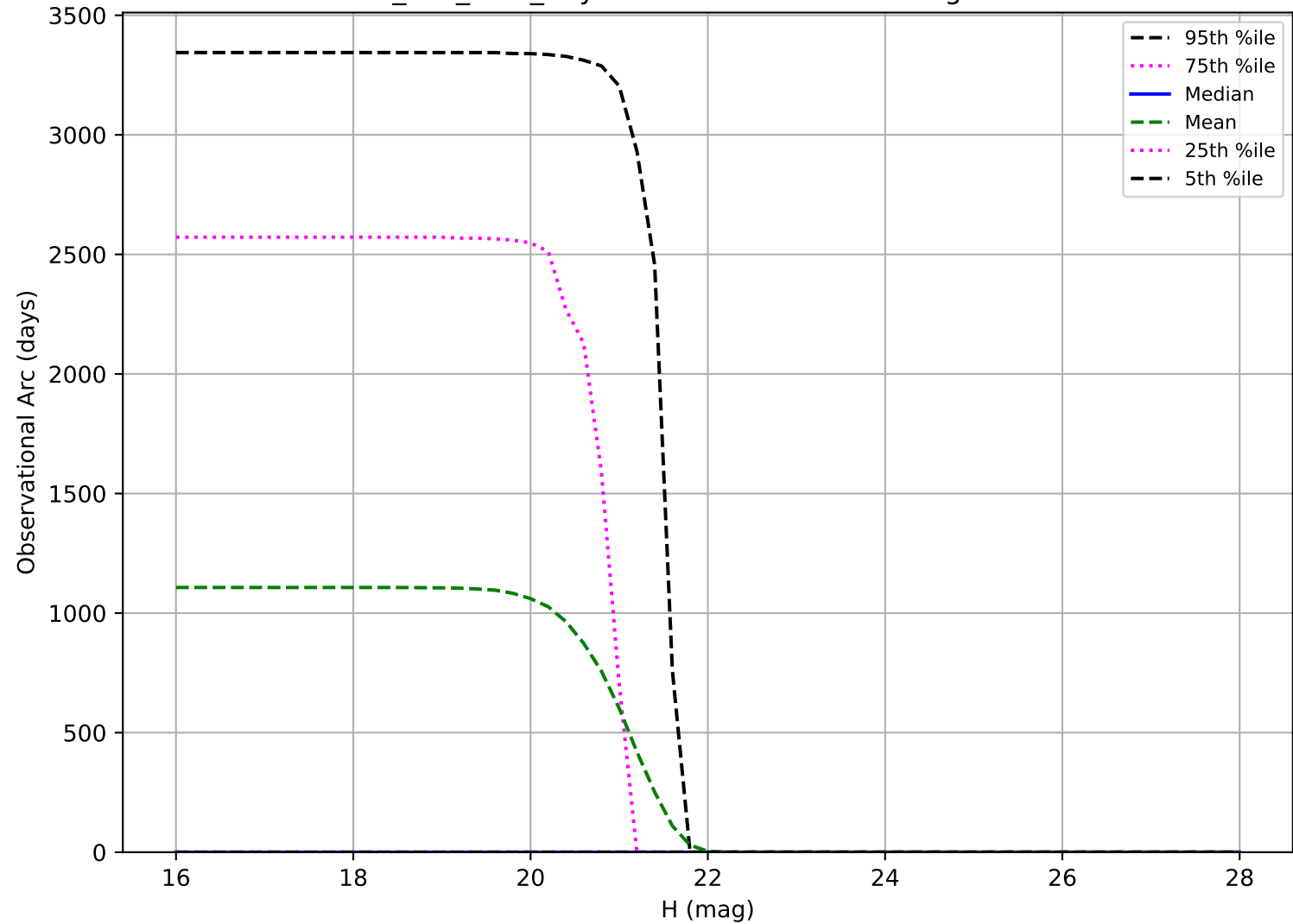
smc_Imc_v3.3_10yrs: Observational Arc Length Vatira
