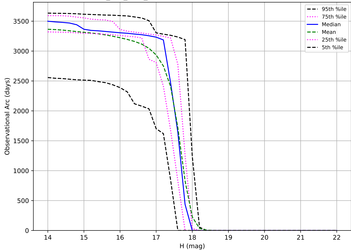
smc_Imc_v3.3_10yrs: Observational Arc Length Trojan
