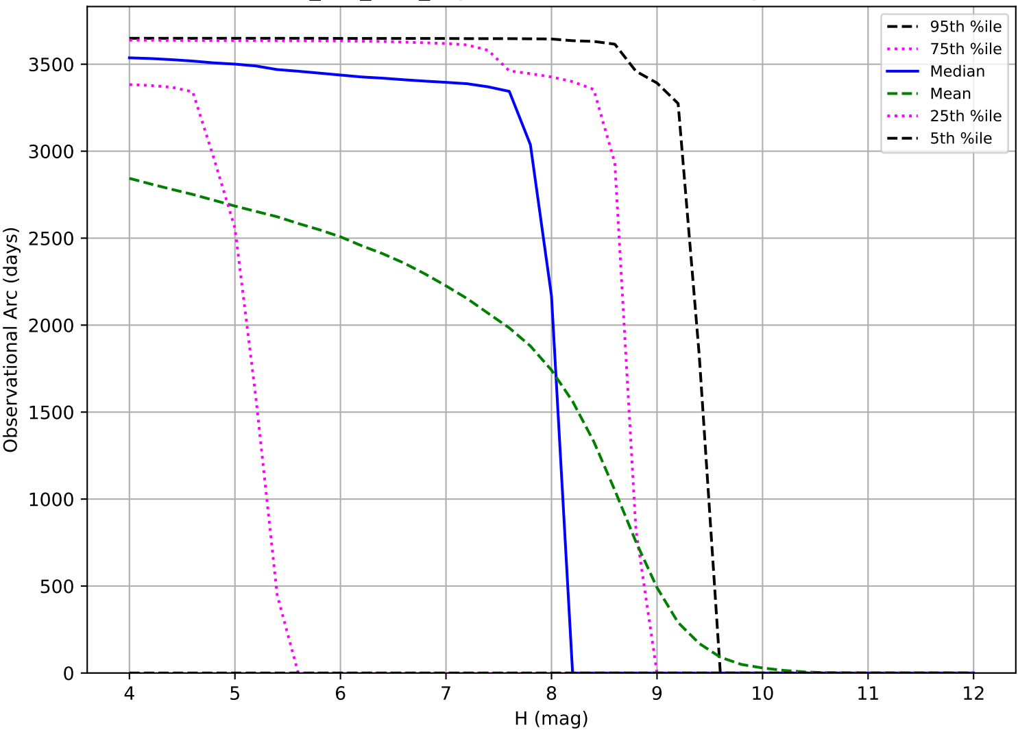
smc_lmc_v3.3_10yrs: Observational Arc Length TNO
