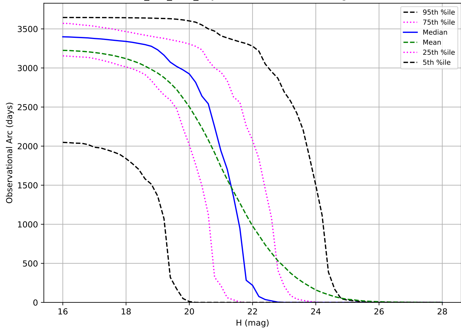
smc_Imc_v3.3_10yrs: Observational Arc Length PHA
