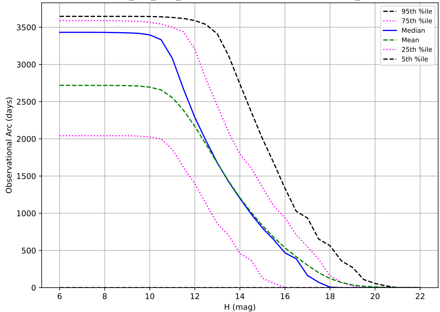
smc_lmc_v3.3_10yrs: Observational Arc Length OCC_r5
