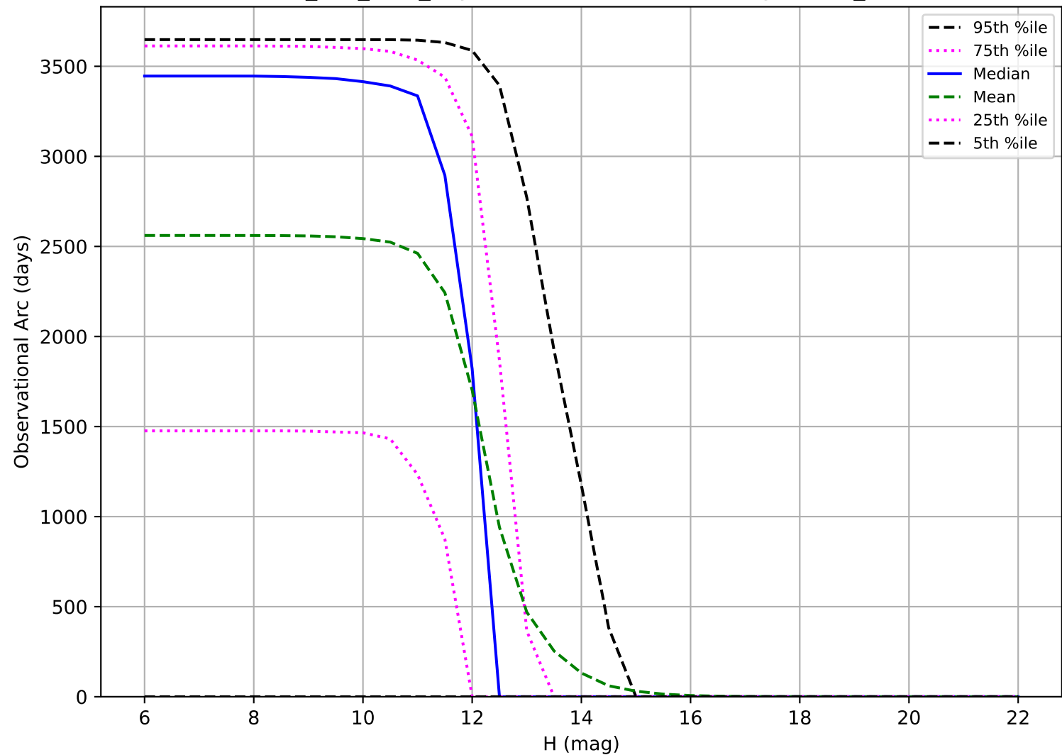
smc_lmc_v3.3_10yrs: Observational Arc Length OCC_r20
