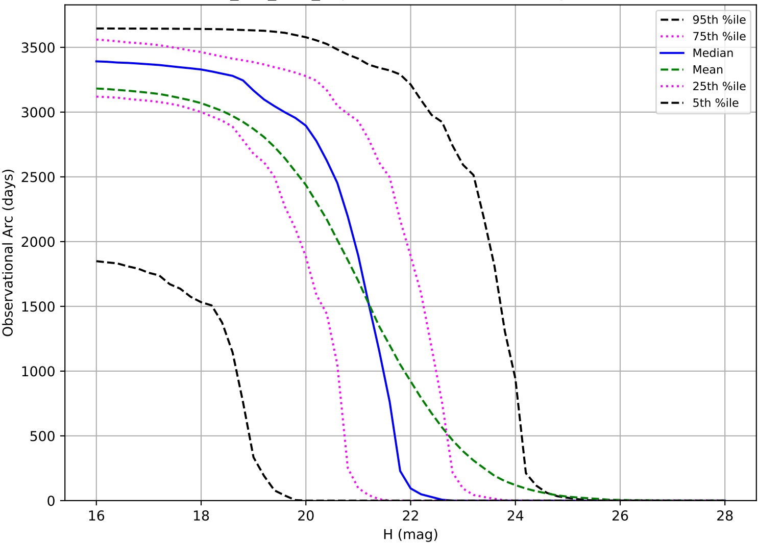
smc_lmc_v3.3_10yrs: Observational Arc Length NEO
