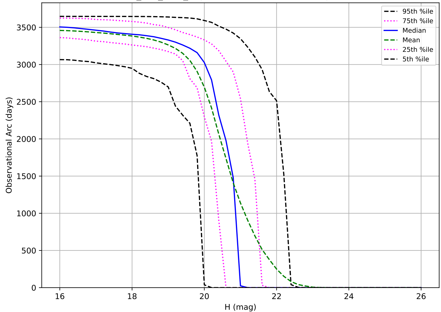
smc_lmc_v3.3_10yrs: Observational Arc Length MBA
