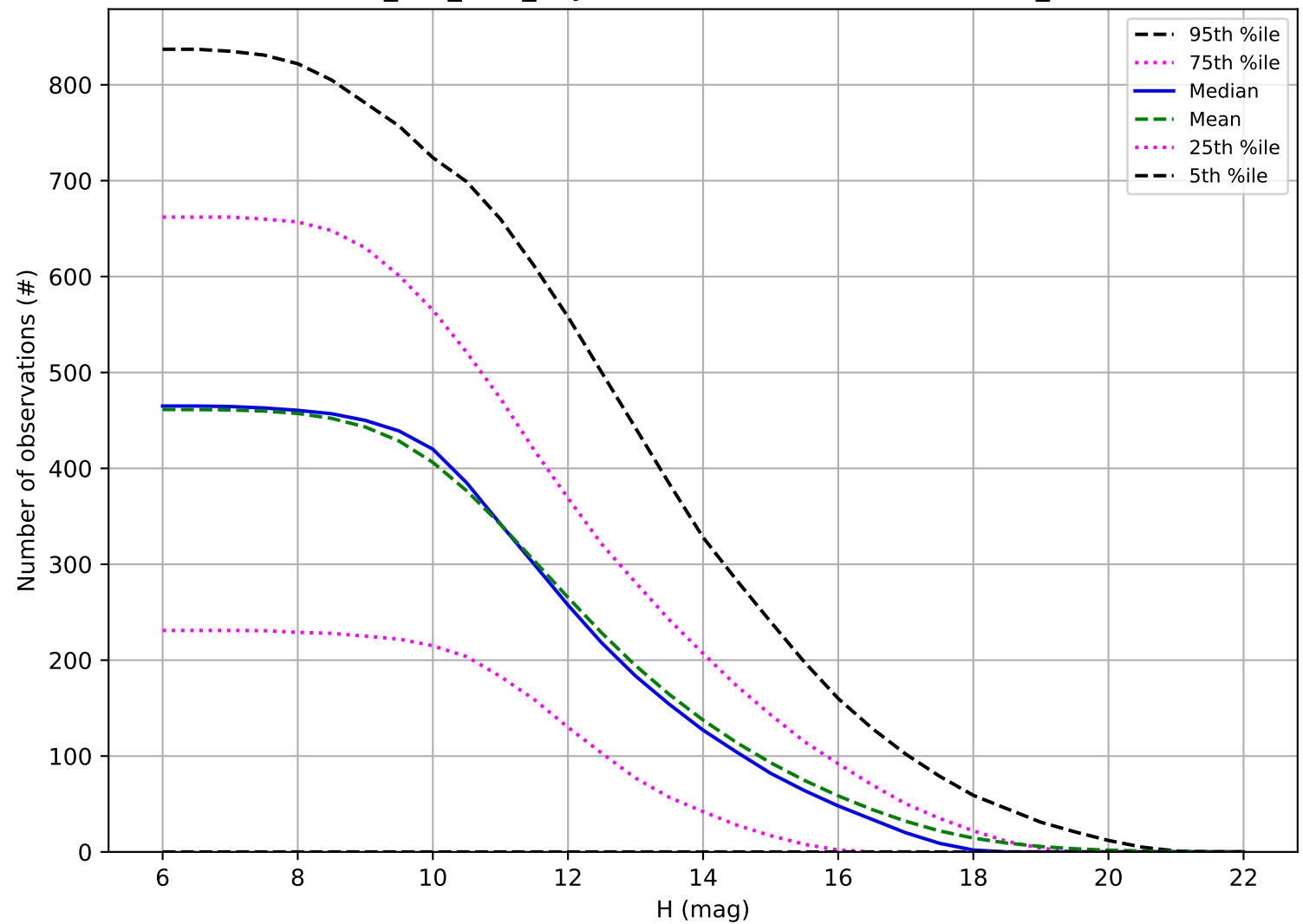
smc_lmc_v3.3_10yrs: Number of observations OCC_r5
