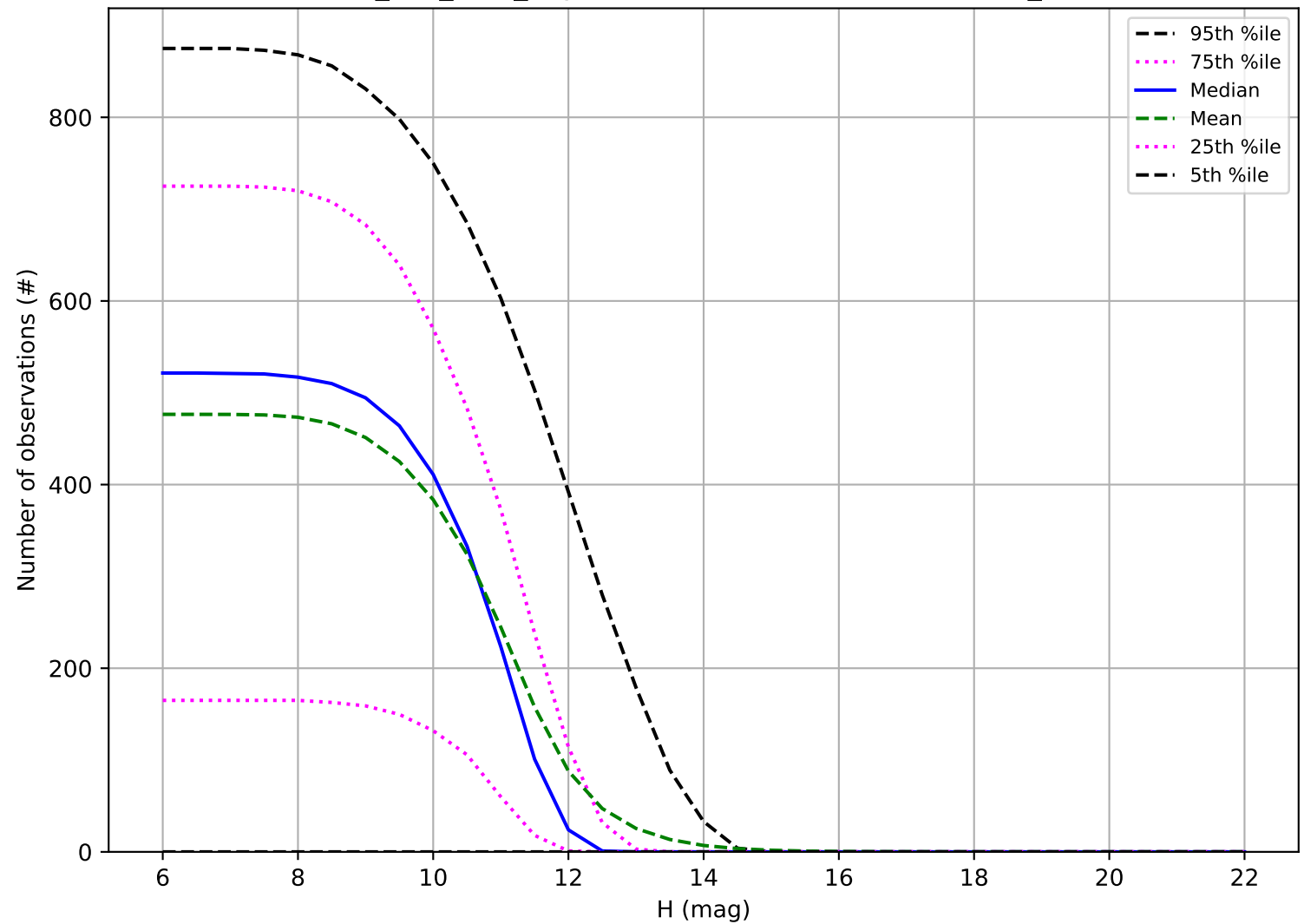
smc_lmc_v3.3_10yrs: Number of observations OCC_r20
