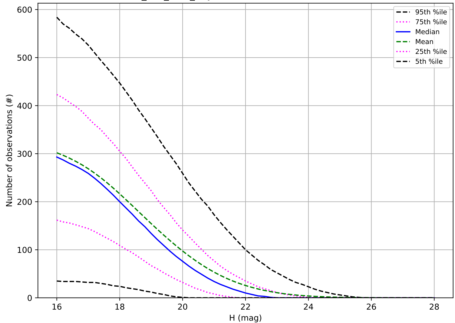
smc_lmc_v3.3_10yrs: Number of observations NEO
