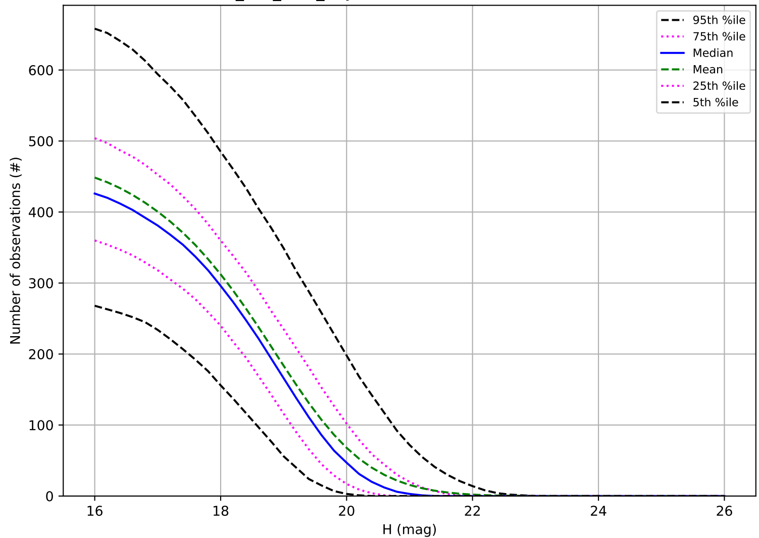
smc_lmc_v3.3_10yrs: Number of observations MBA
