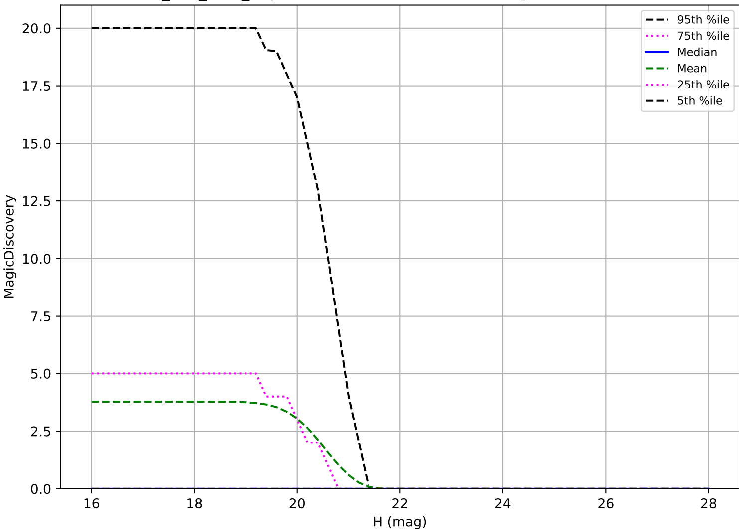
smc_lmc_v3.3_10yrs: Vatira 6 detections in 60 nights detection loss
