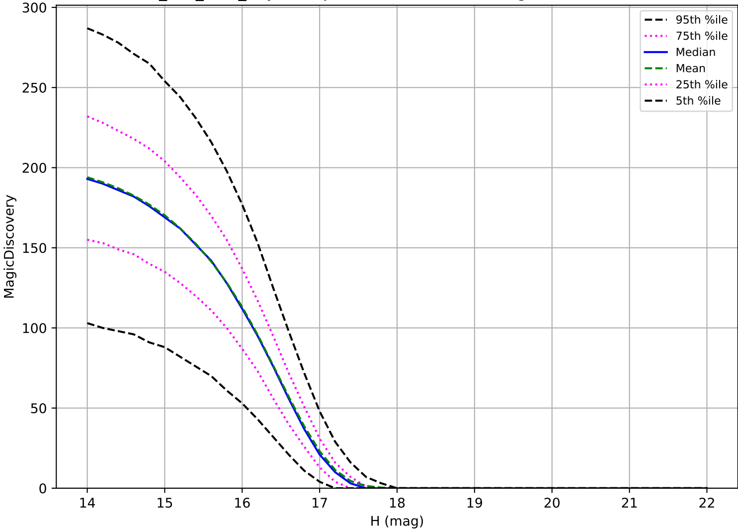
smc_lmc_v3.3_10yrs: Trojan 6 detections in 60 nights detection loss
