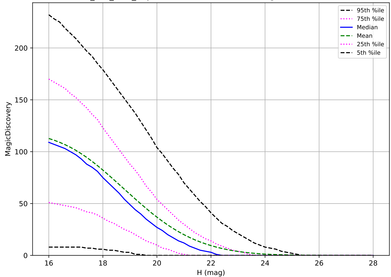
smc_lmc_v3.3_10yrs: PHA 6 detections in 60 nights detection loss
