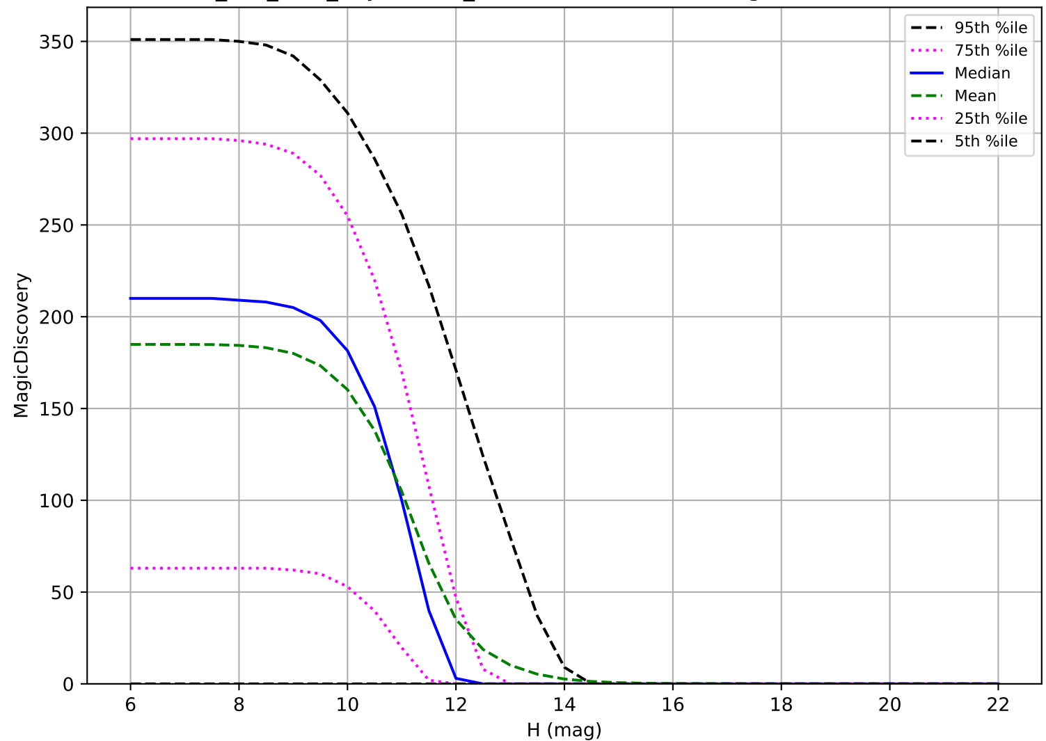
smc_lmc_v3.3_10yrs: OCC_r20 6 detections in 60 nights detection loss
