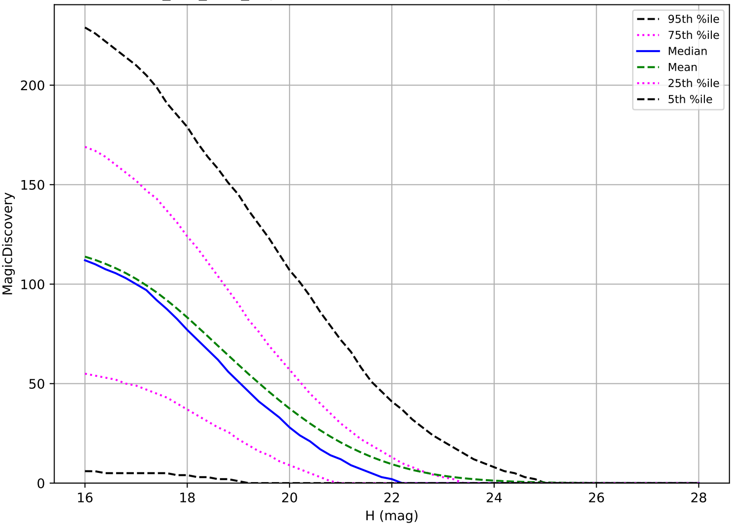
smc_lmc_v3.3_10yrs: NEO 6 detections in 60 nights detection loss
