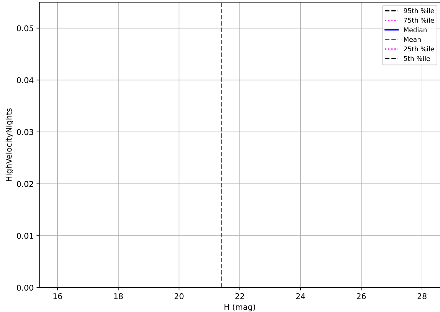
smc_lmc_v3.3_10yrs: Vatira High velocity pair detection loss
